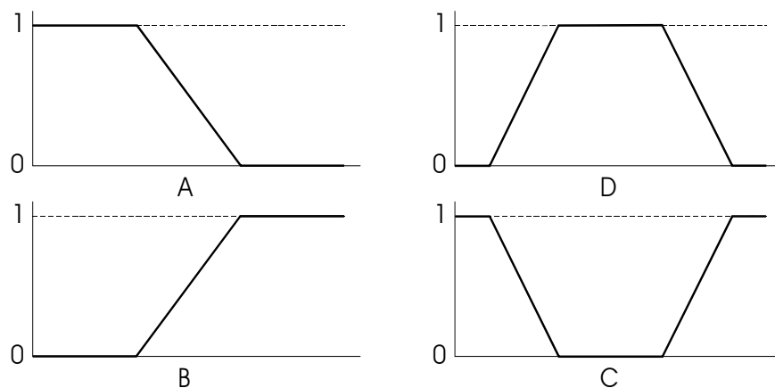
Fig. 1. Fuzzy functions
